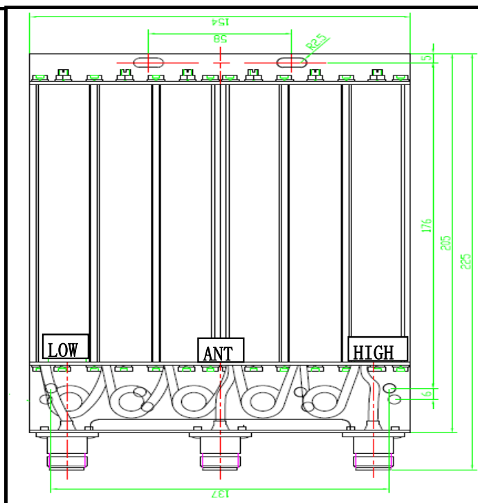
External Drawing
